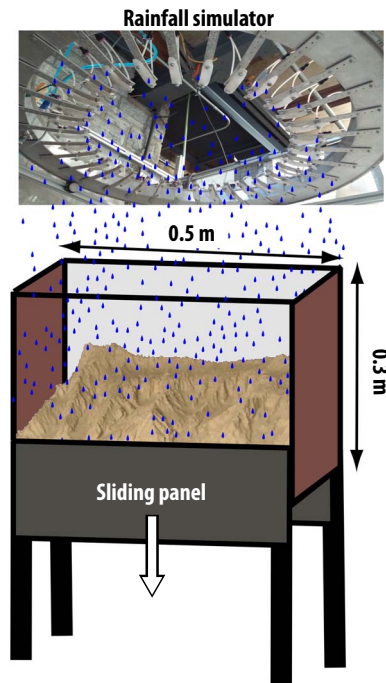
Fig. 1. Schematic representation of the XLE facility at St. Anthony Falls Laboratory, University of Minnesota.
